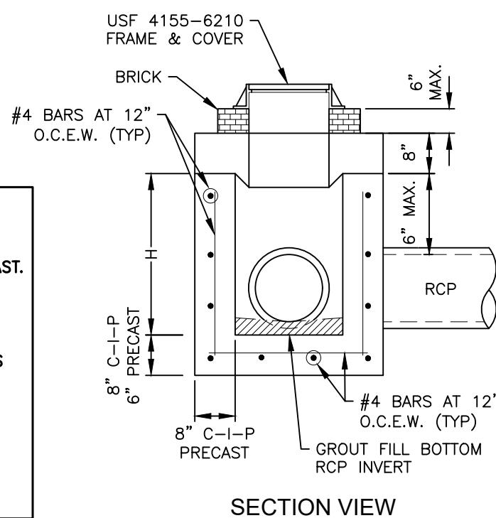
CATCH BASIN DETAIL
