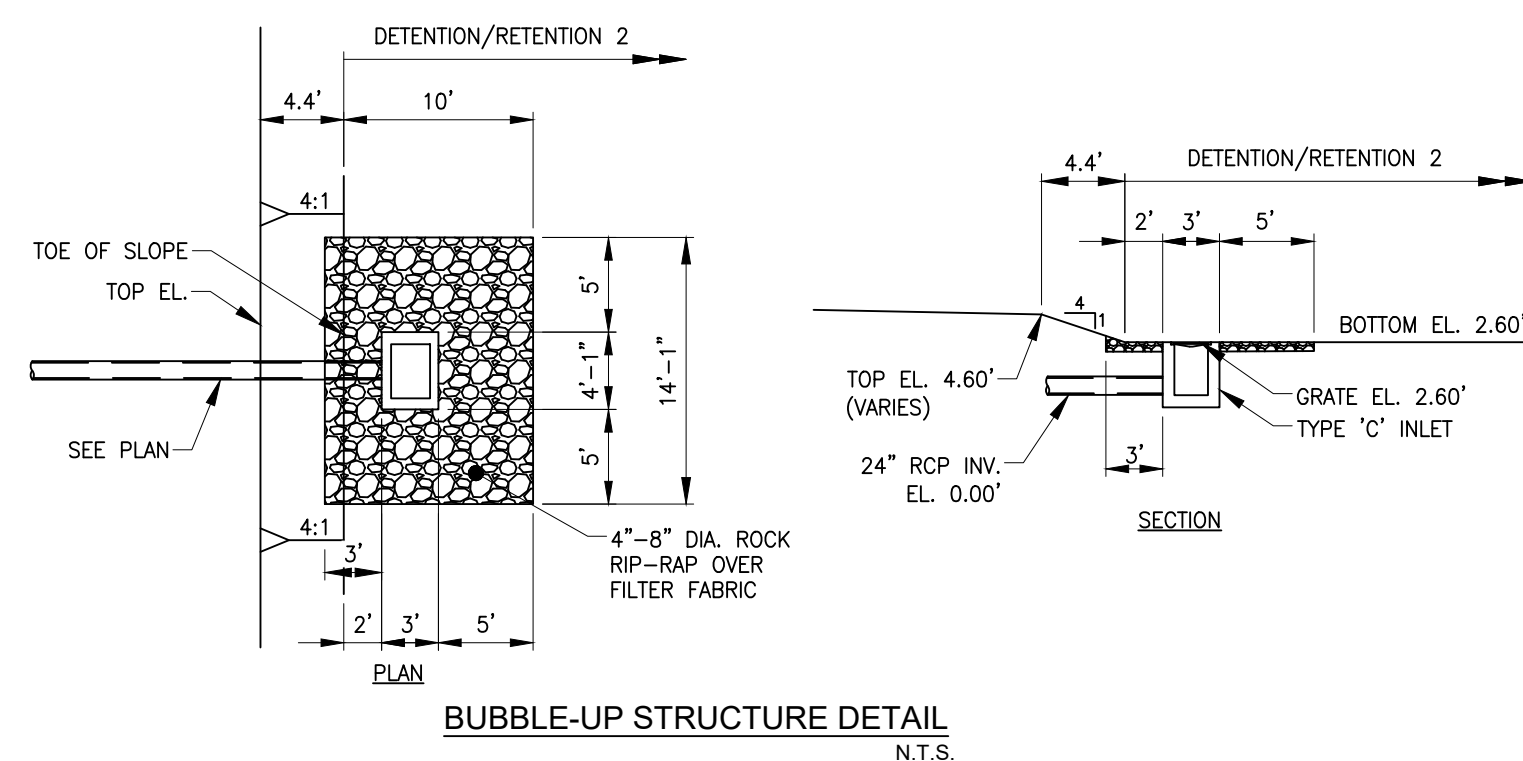
BUBBLE-UP STRUCTURE DETAIL
