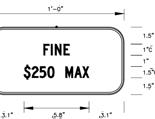
ACCESSIBLE SIGN DETAIL
