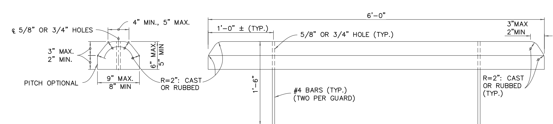
CONCRETE BUMPER GUARD NTS
