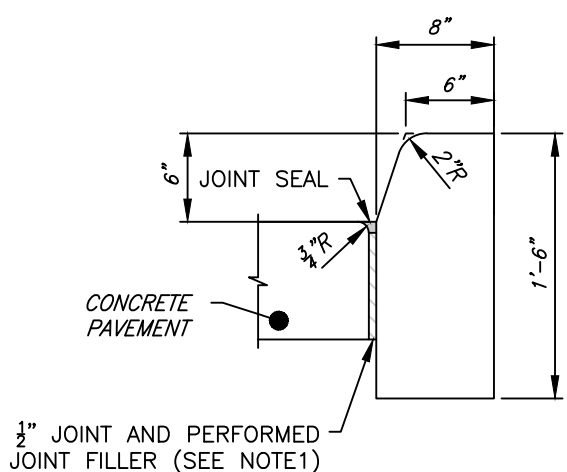
TYPE 'D' CURB DETAIL NTS
