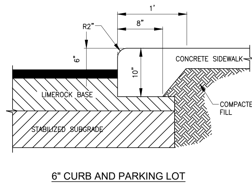
6" CURB AND PARKING LOT NTS
