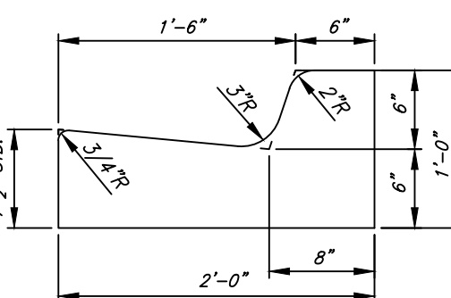
TYPE 'F' CURB DETAIL NTS
